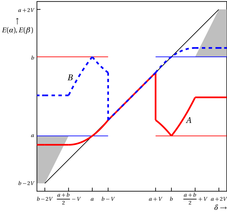
FIGURE 3. The candidates' expected positions across constituencies for V = \frac{1}{3} and (a, b) = (\frac{7}{24}, \frac{17}{24}) .
