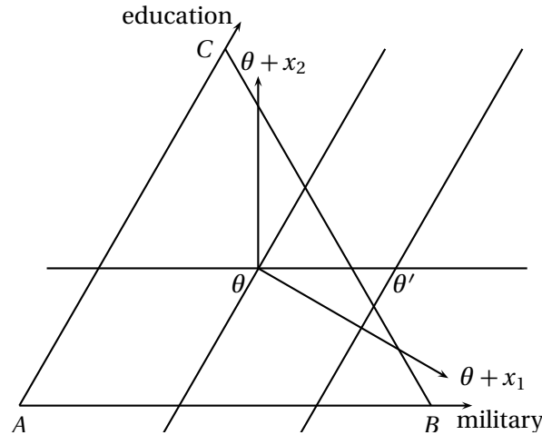
FIGURE 1. Nonnegativity constraints.
