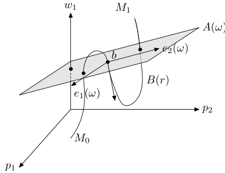
FIGURE 2. Orientation of A(\omega) and B(r) at b .
