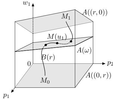
FIGURE 1. The submanifolds A(\omega) and B(r) .
