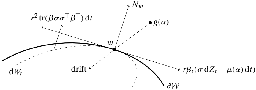
FIGURE 1. At every point w \in \partial\mathcal{W} , the tangential diffusion r\beta_t(\sigma dZ_t - \mu(\alpha) dt) leads to an outward-pointing drift of order r^2 \text{tr}(\beta\sigma\sigma^\top\beta^\top) dt . For sufficiently small r , this term is dominated by the inward-pointing drift r(W_t - g(A_t)) dt .
