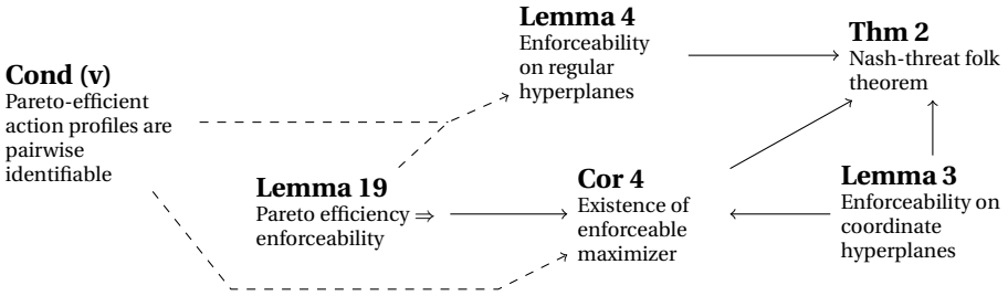
FIGURE 7. Condition (v) enables a shortcut to establish a Nash-threat folk theorem. Lemmas 9, 10 and their preliminary results are still needed, but are not reproduced in this figure to avoid repetition.
