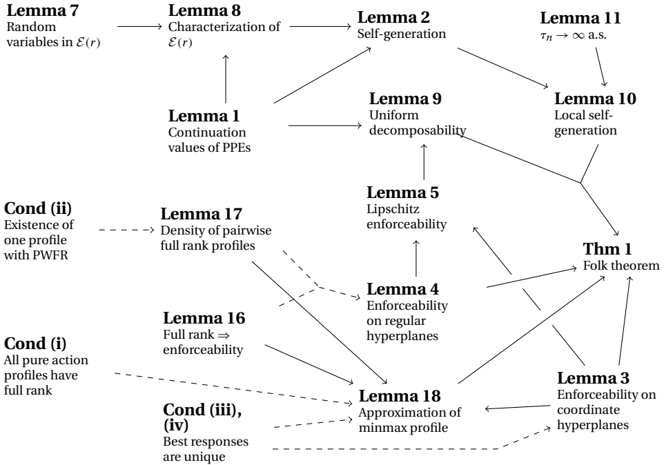
FIGURE 6. Solid arrows indicate the use in the proof; dashed arrows represent sufficient conditions for a result to apply in the proof of Theorem 1 . To establish a Nash-threat folk theorem, Lemma 18 is not needed; hence we can either assume conditions (ii) and (iv) and proceed as above or assume that Pareto-efficient pure action profiles are pairwise identifiable and use the shortcut as in Figure 7 .
