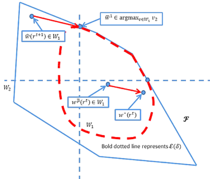
FIGURE 4. The vector from w^{\hat{\mu}}(r^t) to w^*(r^t) is parallel to the one from \hat{w}(r^{t+1}) to \bar{w}^1 .
