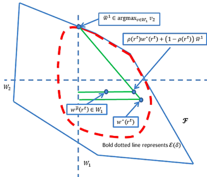
FIGURE 5. \rho(r^t)w^*(r^t) + (1 - \rho(r^t))\bar{w}^1 and w^{\hat{\mu}}(r^t) have the same value for player 2.
