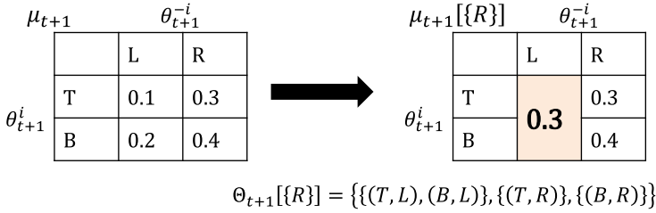
FIGURE 1. An example of \Theta_{t+1}[B_{t+1}^{-i}] and \mu_{t+1}[B_{t+1}^{-i}] ; \Theta_{t+1}^i = \{T, B\} , \Theta_{t+1}^{-i} = \{L, R\} , and B_{t+1}^{-i} = \{R\} .
