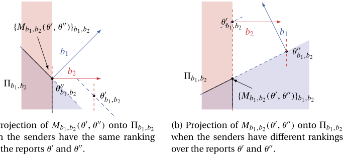
FIGURE 4. Projection of M_{b_1, b_2}(\theta', \theta'') onto \Pi_{b_1, b_2} .
