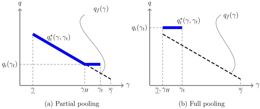
FIGURE 3. The truncated cap allocation, q_i^*(\gamma|\gamma_t) .
