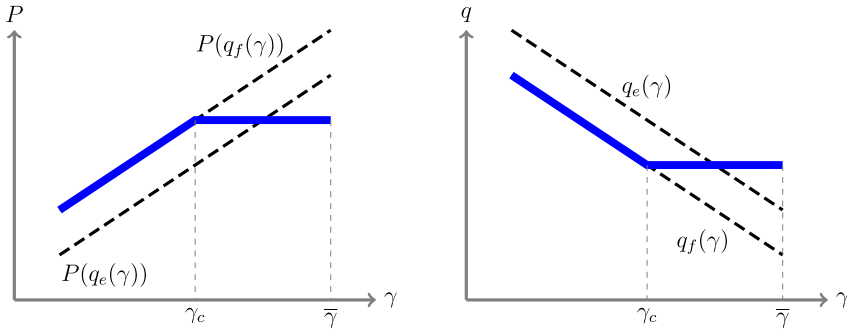
FIGURE 1. Optimal simple cap allocation fails IR.
