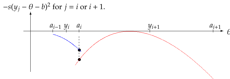
FIGURE 2. x_{i+1} > x_i + 4b .
