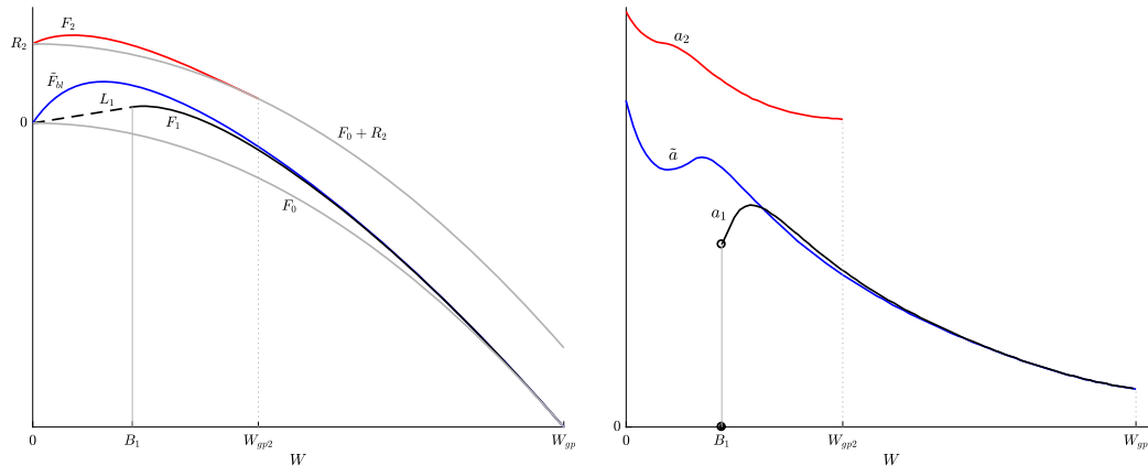
FIGURE 3. Optimal solution curves and their associated effort policy functions in three examples. Baseline example with B = R = 0 : solution curve \tilde{F}_{\text{bl}} (left panel) and its effort policy function \tilde{a} (right panel). Example E_1 with B = B_1 > 0 and R = 0 : solution L_1 spliced with F_1 , and the associated effort policy function a_1 (discontinuous at B_1 ). Example E_2 with B = 0 and R = R_2 > 0 : solution F_2 and its effort policy a_2 . Parameter values as in Figures 1 and 2.
