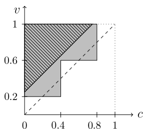
(b) Full information (hatched) and optimal three element information structure (gray shaded).
