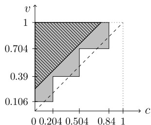
(c) Full information (hatched) and optimal four element information structure (gray shaded).
