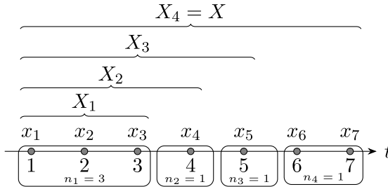
FIGURE 1. A contest with 7 players and 3 disclosures. Players 1 to 3 choose efforts x_1, x_2, and x_3 independently; player 4 observes X_1 = x_1 + x_2 + x_3, player 5 observes X_2 = X_1 + x_4, and players 6 and 7 observe X_3 = X_2 + x_5.
