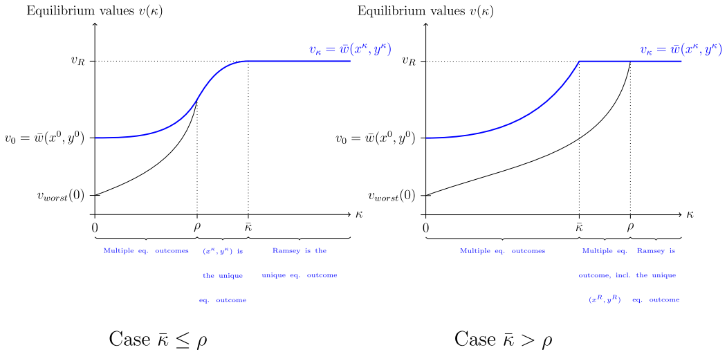
FIGURE 2. Best and worst equilibrium payoffs as a function of \kappa . In the two graphs, we plot the best ( v_\kappa ) and the worst ( v_{\text{worst}} ) equilibrium payoffs for the government as a function of commitment ability ( \kappa ). The left-hand panel corresponds to the case in which \bar{\kappa} —the minimum commitment ability required to achieve the Ramsey outcome—is below the cost of controllability \rho . The right-hand panel corresponds to the case in which \bar{\kappa} is above \rho .
