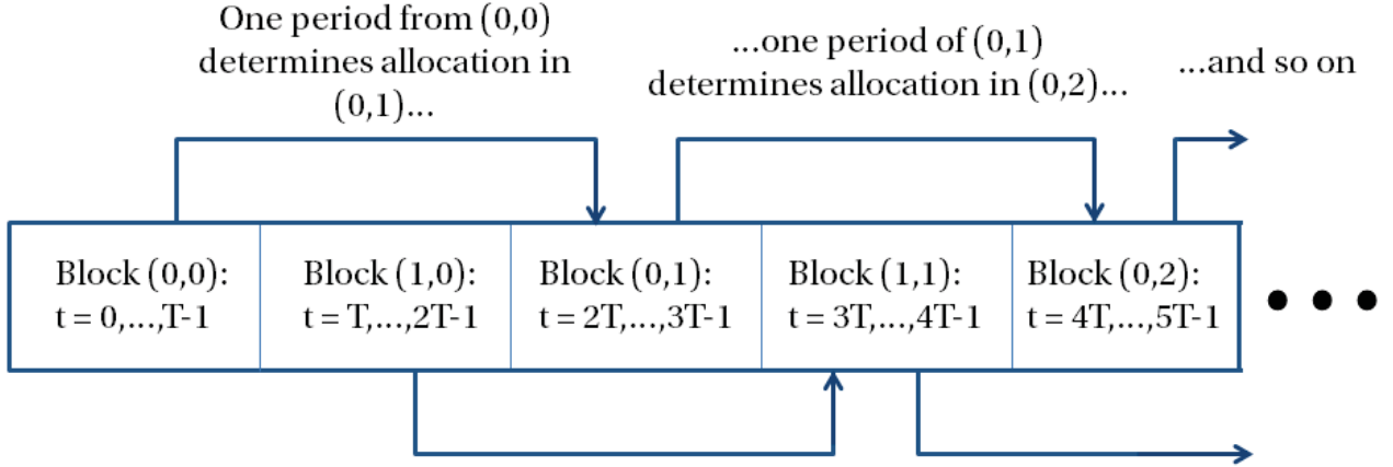
Figure 1: A (T, 2) -Recurrent mechanism. Each block represents T periods. Arrows indicate which periods influence the targeted allocation rule in each block.
