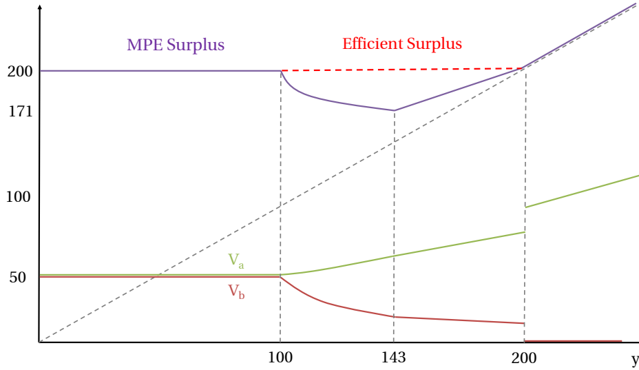
Figure 2: The plot depicts the limiting payoffs, the limiting MPE surplus, and the limiting efficient surplus as a function of s_{ad} = y for Example 1. The payoff of players a and d is denoted by V_a , whereas V_b denotes the payoff of b and c .
