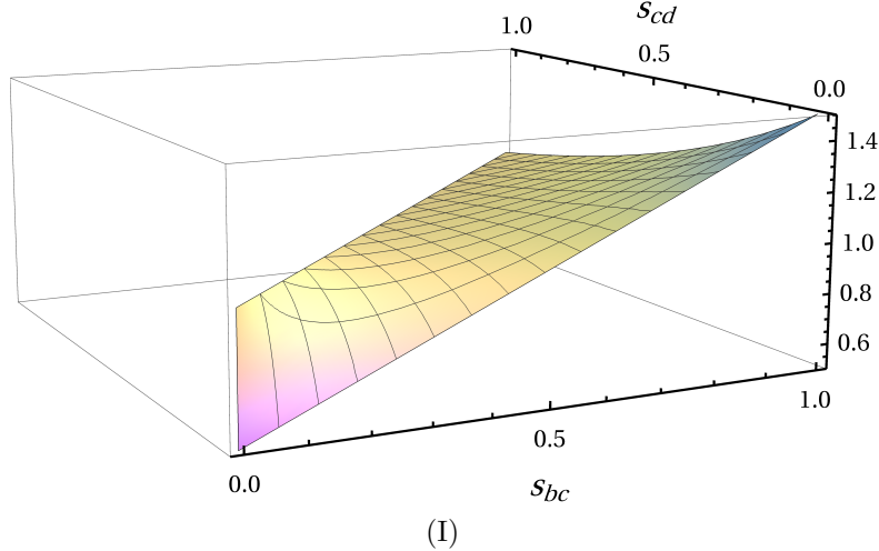
Figure 6: The lower bound for \zeta for different combinations of s_{cd} and s_{bc} is plotted. As \zeta < 1 , regions of the parameter space where lower bound is greater than 1 are regions in which no sequential LMPE exists.
