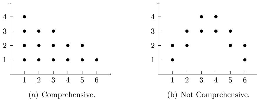
Figure 1: Sets in \mathbb{N}^2
