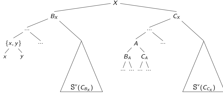
Figure 5: The recursive construction of S^v .
