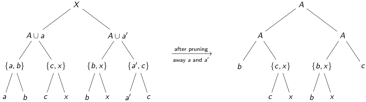
Figure 2: Left: an agenda T on X . Right: the pruned agenda T|_A on A \subset X .
