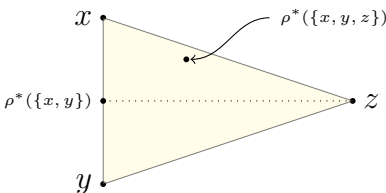
Figure 2: Path independence and Luce's IIA.
