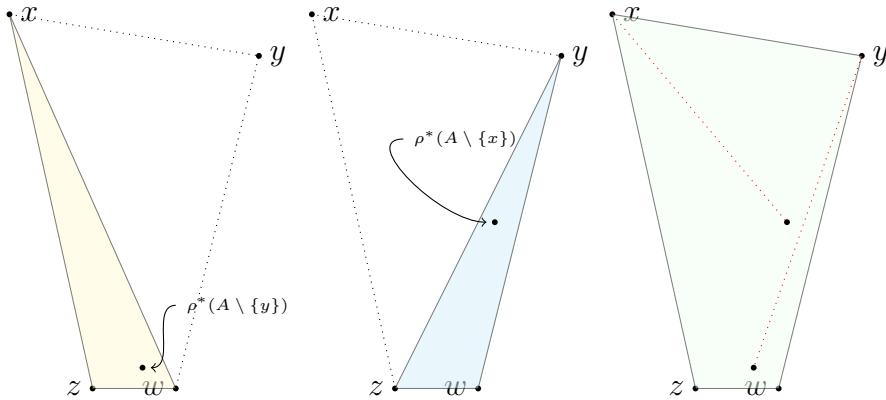
Figure 3: Violation of partial path independence; A = \{x, y, z, w\} .
