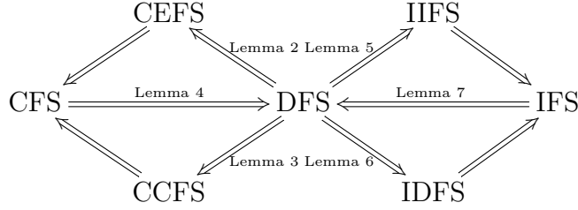
Figure 1: Proof strategy for Theorem A.1. Any unlabeled implication is immediate.
