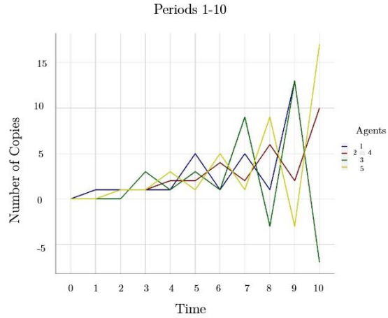
(b) Learning dynamics in this network
