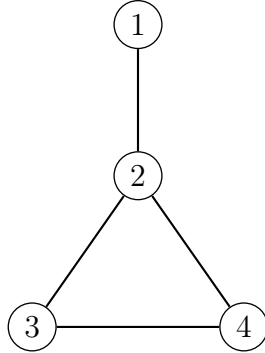
FIGURE 5. Long-run inefficient equilibria without link removals
