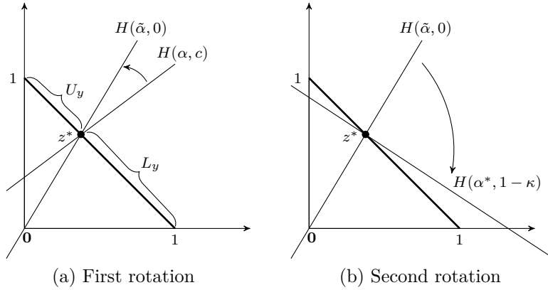
Figure 5: Separating hyperplanes.
