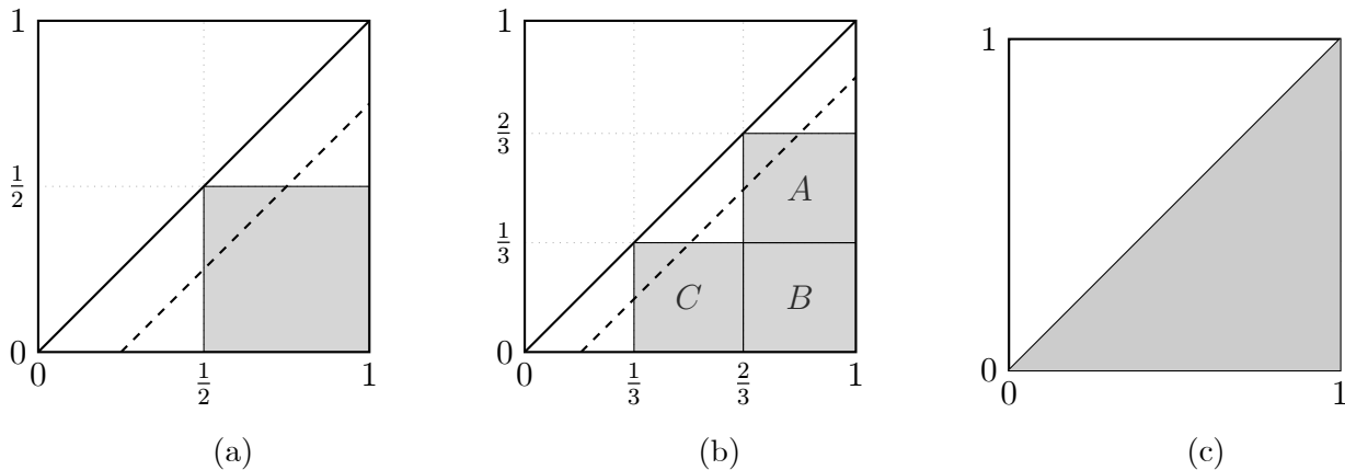
Figure 5: Bilateral trade with uniform distributions and a subsidy.
