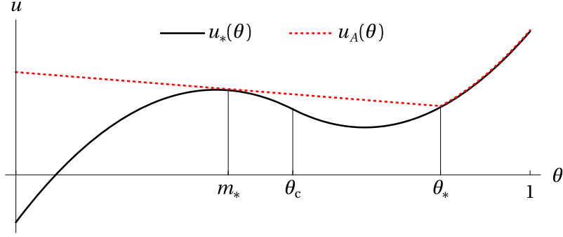
Figure 2: Joint and auxiliary payoff functions
