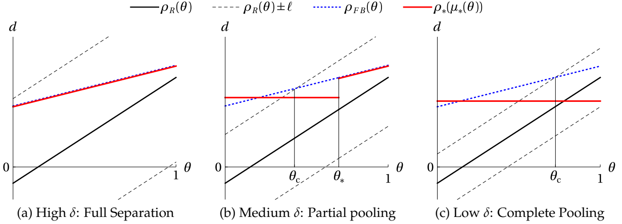
Optimal decision rules and decision outcomes given a highly-responsive, downward-biased receiver. Figure 3a shows the high- \delta case, with full separation and \theta_c = \theta_* = 0 ; Figure 3b shows the intermediate- \delta case, with partial pooling and 0 < \theta_c < \theta_* < 1 ; Figure 3c shows the low- \delta case, with complete pooling and 0 < \theta_c < \theta_* = 1 . The last two cases illustrate overpooling: \theta_c < \theta_* .
