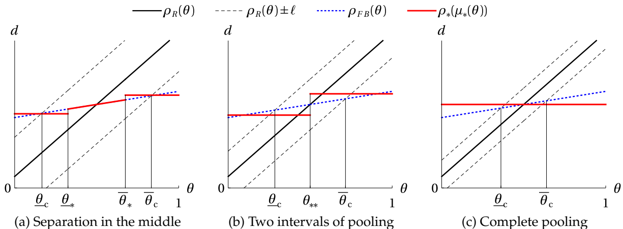
Optimal decision rules and decision outcomes given a highly-responsive receiver and two intervals of high-conflict states, [0, \underline{\theta}_x) and (\bar{\theta}_x, 1] . Figure 4a shows the case of relatively high \delta , with two pooling intervals [0, \underline{\theta}_*) and (\bar{\theta}_*, 1] and separation of the middle states \theta \in (\underline{\theta}_*, \bar{\theta}_*) . Figure 4b shows the intermediate- \delta case, with two adjacent pooling intervals [0, \theta_{**}) and [\theta_{**}, 1] . Figure 4c shows the low- \delta case with complete pooling. Overpooling occurs in all cases.
