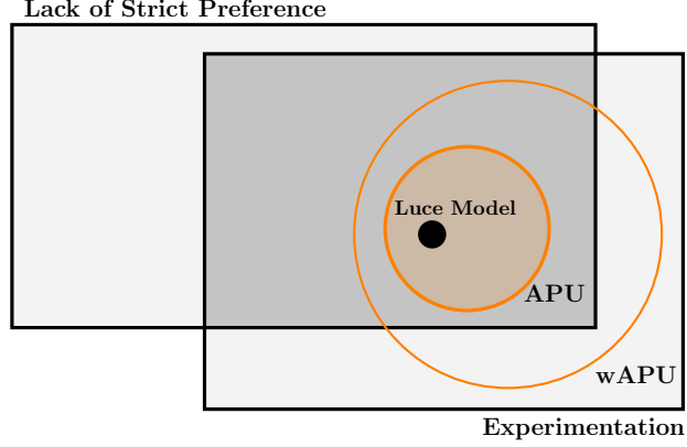
Figure 3: Weak APU, Lack of Strict Preference, and Experimentation
