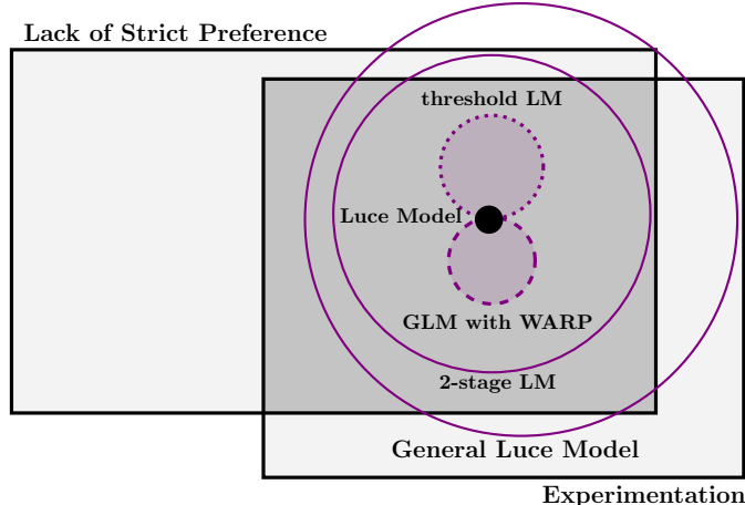
Figure 1: General Luce Model, Lack of Strict Preference, and Experimentation
