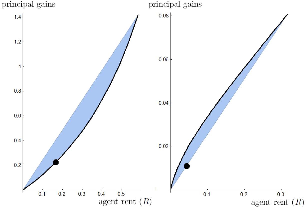
Figure 1: Examples with F/f convex and concave
