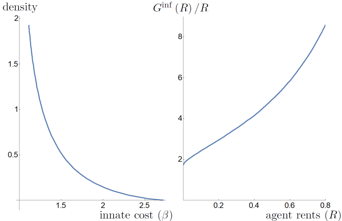
Figure 2: Example based on Gagnepain and Ivaldi (2002, Table 3)
