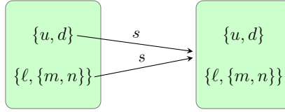
Figure 5: ICP for Type III individuals
