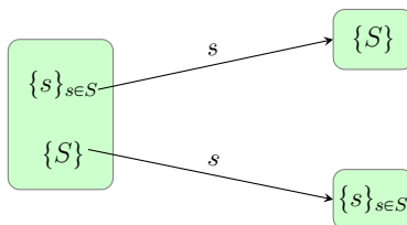
Figure 3: ICP for Type I individuals
