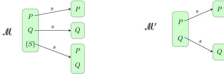
Figure 2: Two-period ICPS, \mathcal{M} and \mathcal{M}'
