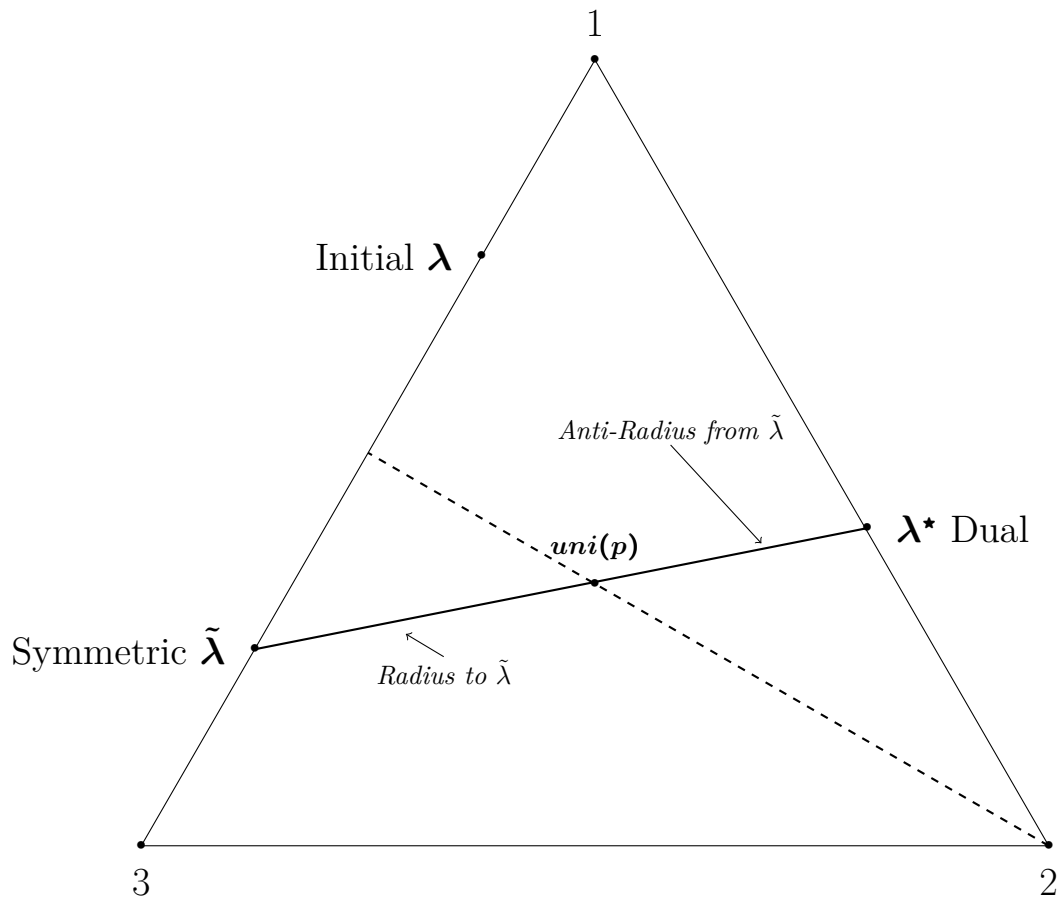
Figure 1: The duality operation
