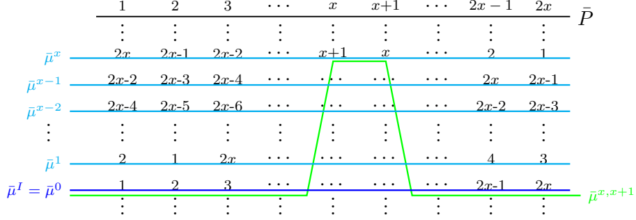
Figure 12: Problem \bar{P} = (\bar{N}, \bar{R}) .
