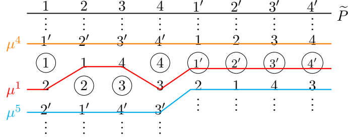
Figure 16: Problem \tilde{P} .
