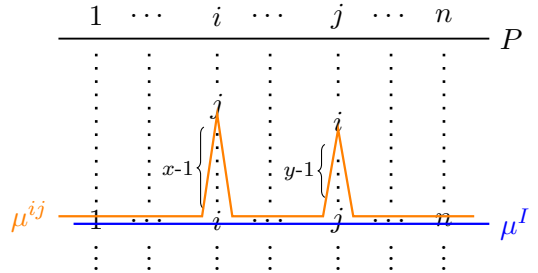
Figure 5: A one-couple matching \mu^{ij} of length (x, y) .
