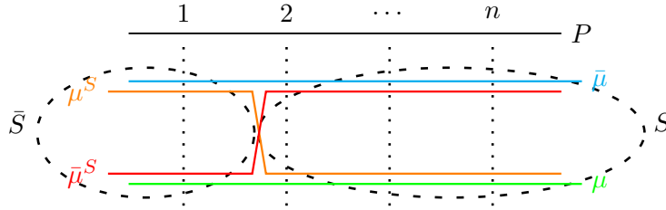
Figure 3: The general view of the Decomposition Lemma.
