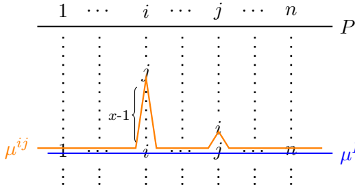
Figure 4: A one-couple matching \mu^{ij} of length (x, 1) .
