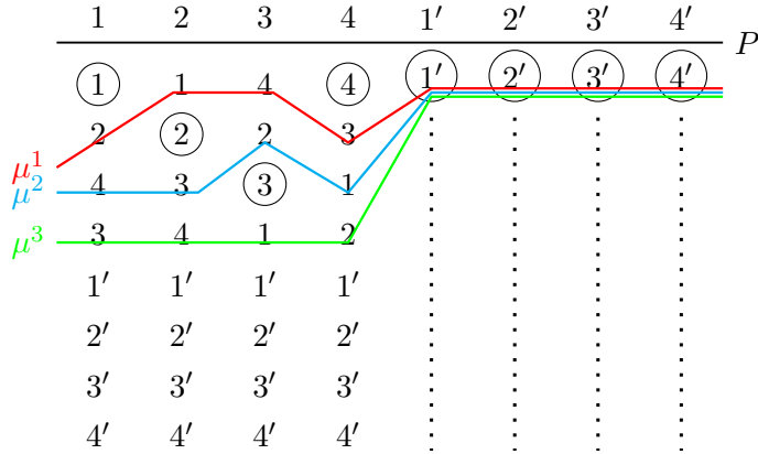
Figure 14: An extension of the problem P in Figure 6 by the set of agents A = \{1', 2', 3', 4'\} .
