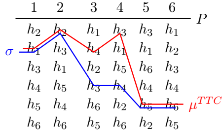
Figure 1: House allocation problem.
