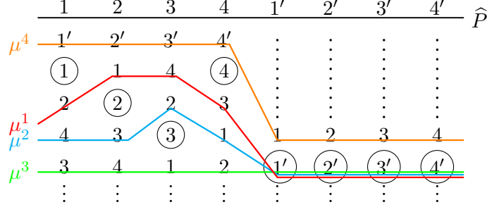
Figure 15: Problem \widehat{P} .
