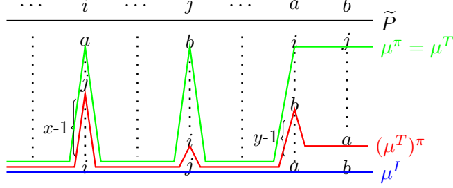
Figure 11: Problem \tilde{P} , after swapping the positions of \mu^\pi and (\mu^T)^\pi in problem \hat{P}^\pi in Figure 10.
