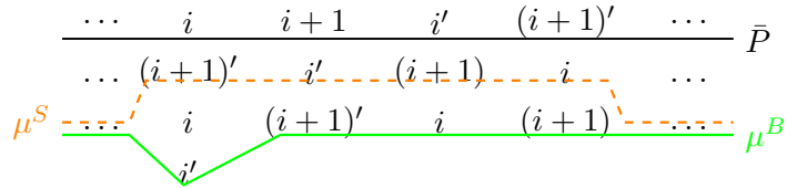
Figure 22: The one singleton structure with i as the singleton.
