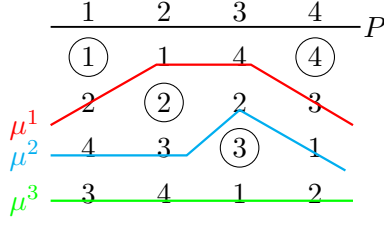
Figure 6: A problem over four agent with one singleton agent between the matchings.
