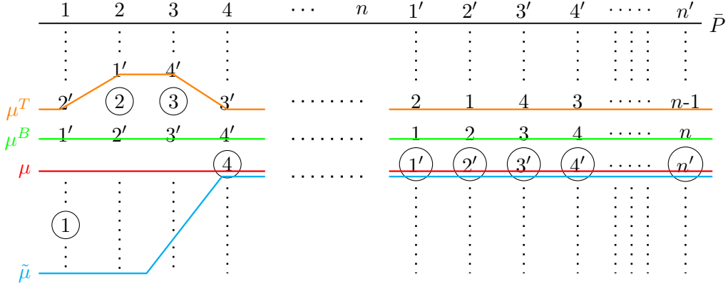
Figure 20: General structure for \bar{P} .
