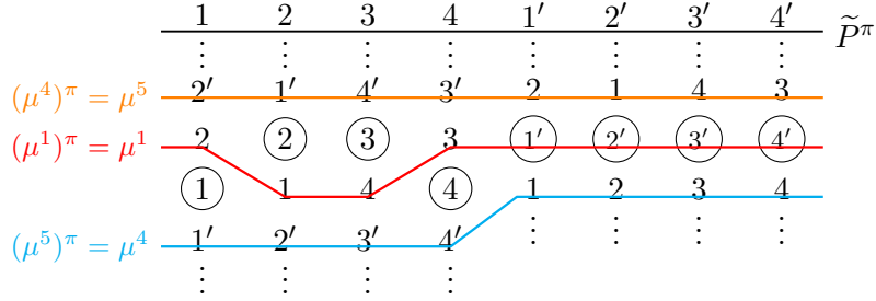
Figure 17: Problem \tilde{P}^\pi after permuting \tilde{P} in Figure 16 with \pi = (12)(34) .
