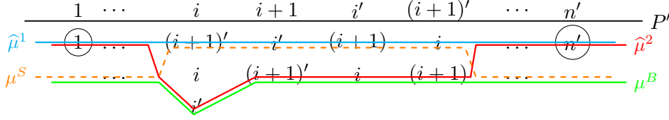
Figure 24: The problem P' .
