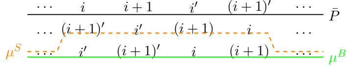
Figure 21: The no singleton structure.
