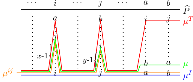
Figure 9: Problem \widehat{P} = (\widehat{N}, \widehat{R}) .
