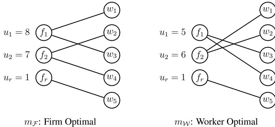
FIGURE 1. Stable Matchings
