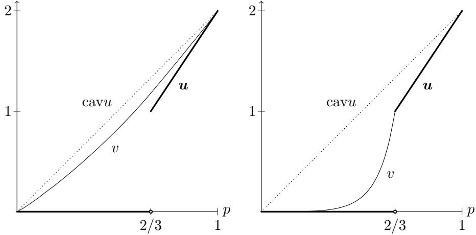
(a) Evidence accumulates rapidly. (b) Evidence accumulates slowly.
