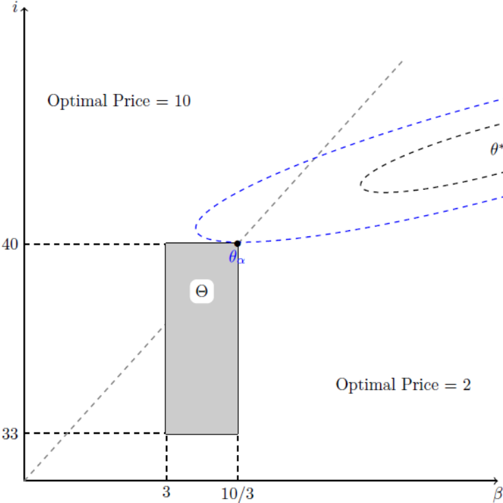
Figure 2: The ellipses are the KL-level curves in the equilibrium of part b where \psi(2) = 35/36 .
